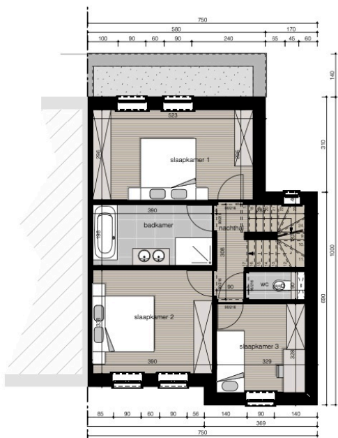
VERDIEPING +1 1/100
